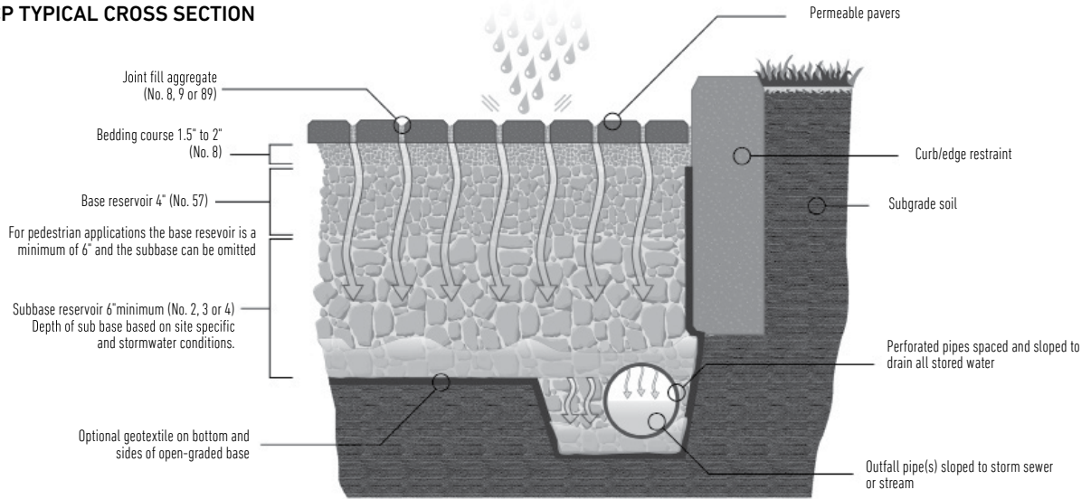
PICP TYPICAL CROSS SECTION
