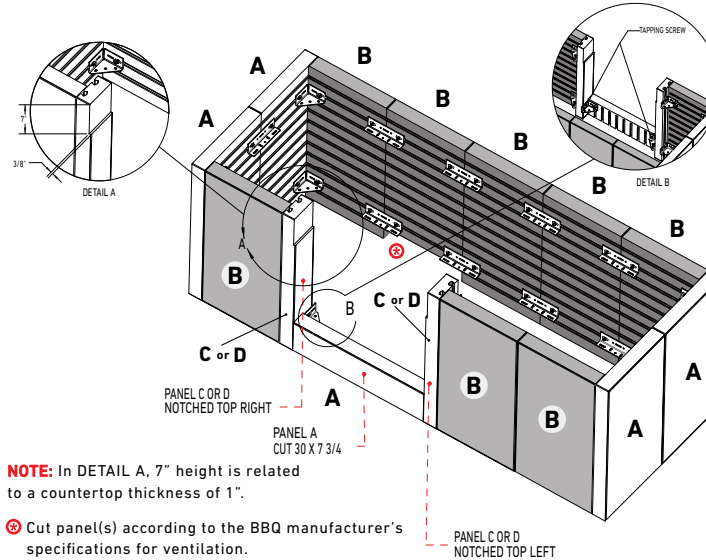
VISTA INTERIOR
